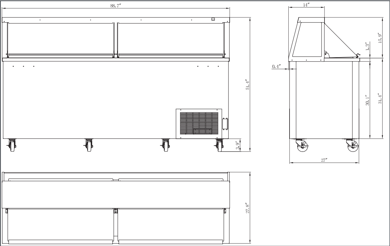
BMAD System (Low maintenance high performance). Dimensions rounded up to the nearest inch or millimeter. Specifications subject to change without notice.
