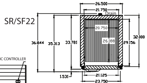
Plan Views
