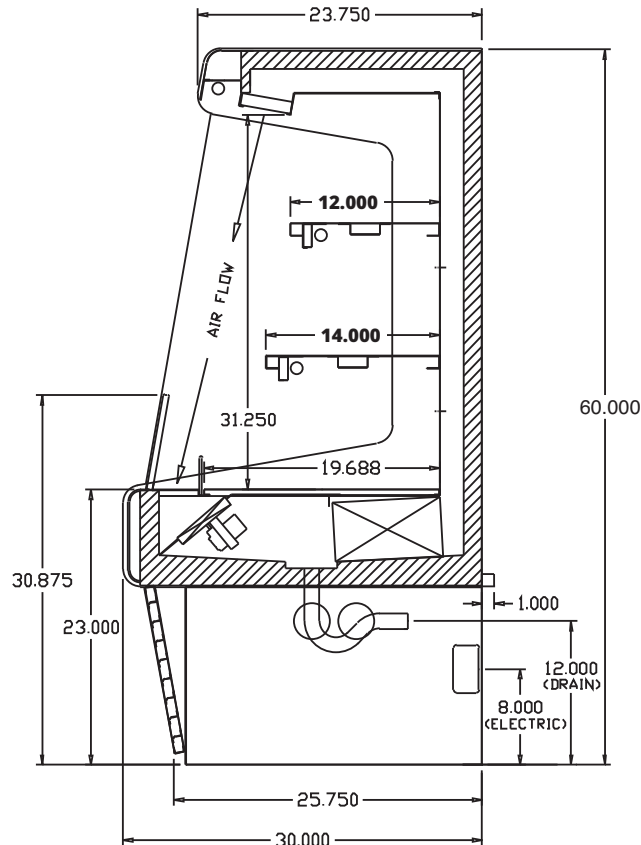
CROSS SECTION
