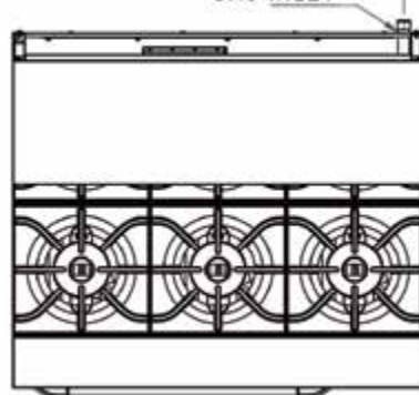
TOP VIEW 3/4" NPT GAS INLET 1 11/16"
